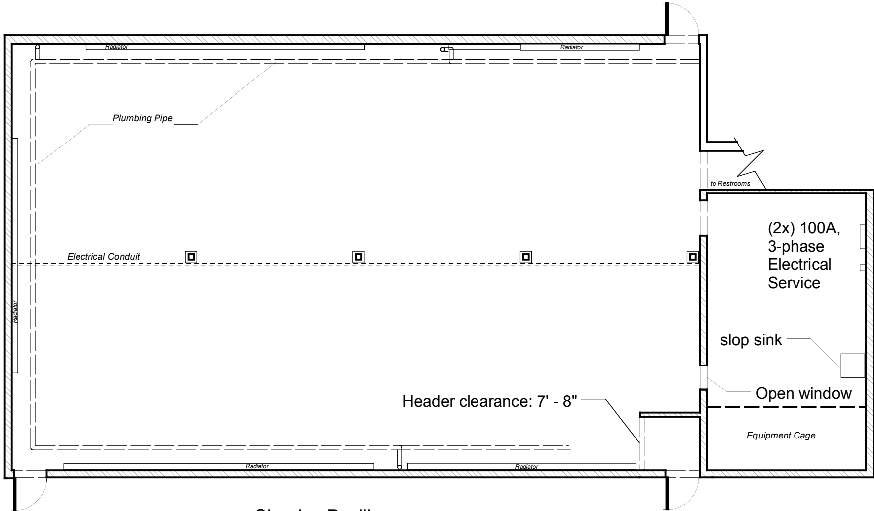
Shanley Pavilion Norris University Center Northwestern University Scale: 1/8" = 1' - 0" Last Update: 6/6/03
